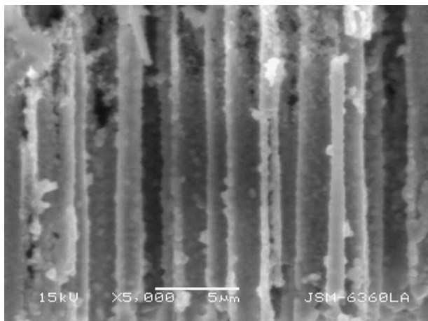
Fig. 3. Magnified pictures of the cross-sectional SEM images of the microstructure of the Ni–Pd/silicon MCP after electrochemical measurements.
