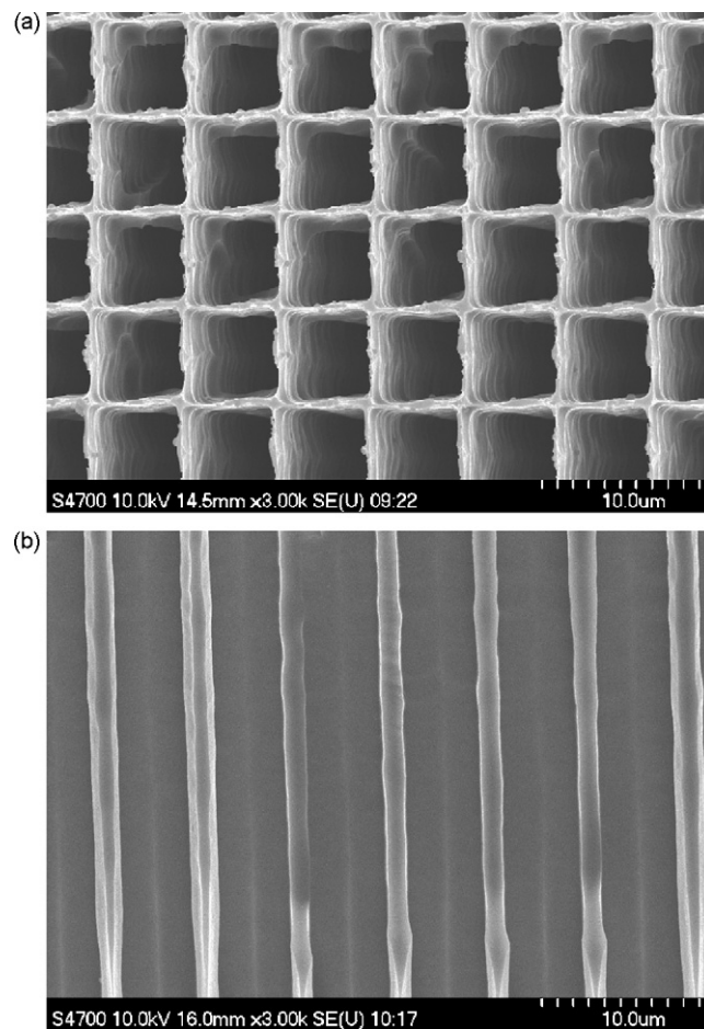
Fig. 1. (a) Top and (b) cross-sectional SEM images of the microstructure of the silicon MCP.
