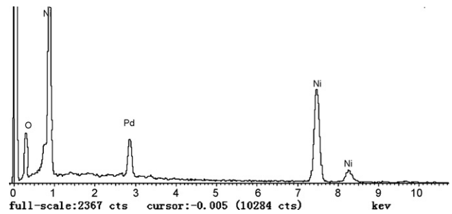
Fig. 4. Corresponding EDS image of the structure in Fig. 3.
