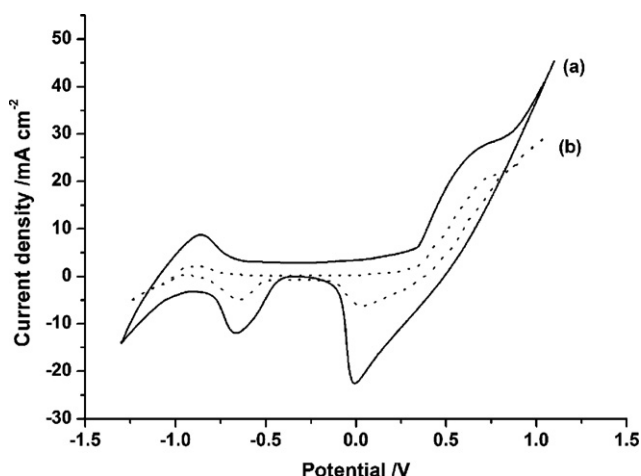
Fig. 6. Cyclic voltammograms of the Ni–Pd/Si–MCP (a) and Ni–Pd/Si (b) composite in 2.0 M KOH aqueous solution with broad potential range at the scan rate of 50 \text{ mV s}^{-1} .
