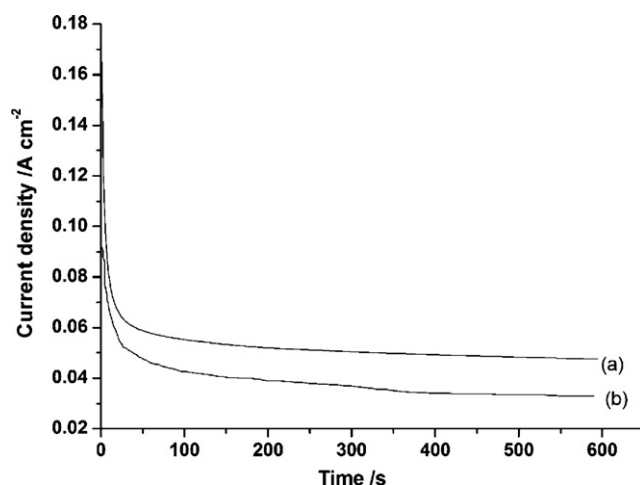
Fig. 7. Chronoamperogram of electroactivity of (a) Ni–Pd/Si–MCP and (b) Ni–Pd/Si electrode at an oxidation potential -0.4 \text{ V} for methanol electro-oxidation in the 2 M KOH and 1 M methanol aqueous solution at 25^\circ\text{C} .
