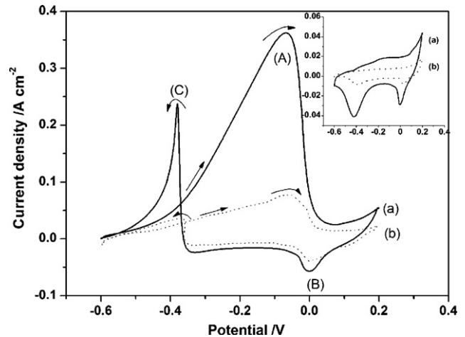
Fig. 5. Cyclic voltammograms of the Ni–Pd/Si–MCP (a) and Ni–Pd/Si (b) composite in 2.0 M KOH aqueous solution with and without methanol (in the inset) at room temperature with the scan rate of 50 \text{ mV s}^{-1} .
